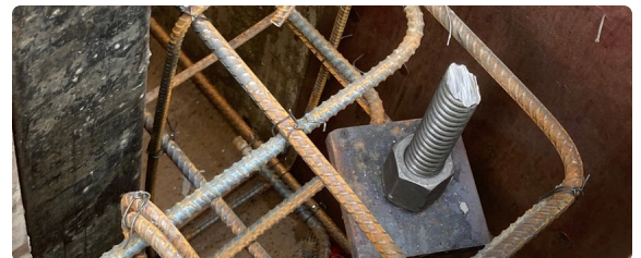
Pile top and bearing plate set in the cap reinforcing.
